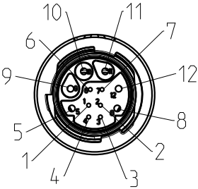
plug face male
