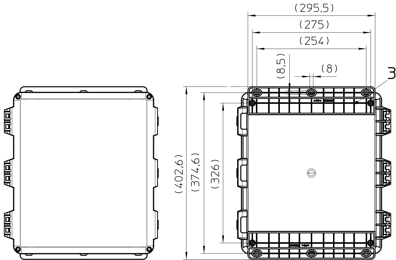
Application with OCS MOUNT 1412 SET
