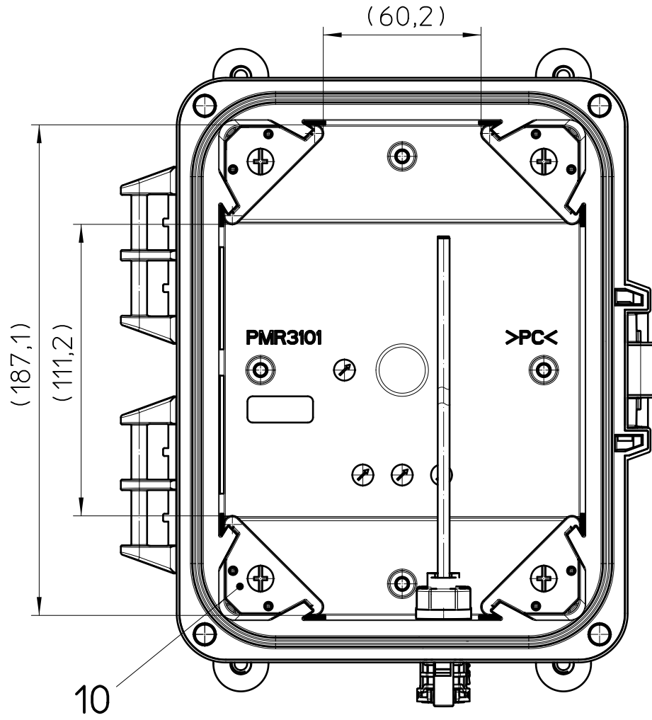
Front view without cover
