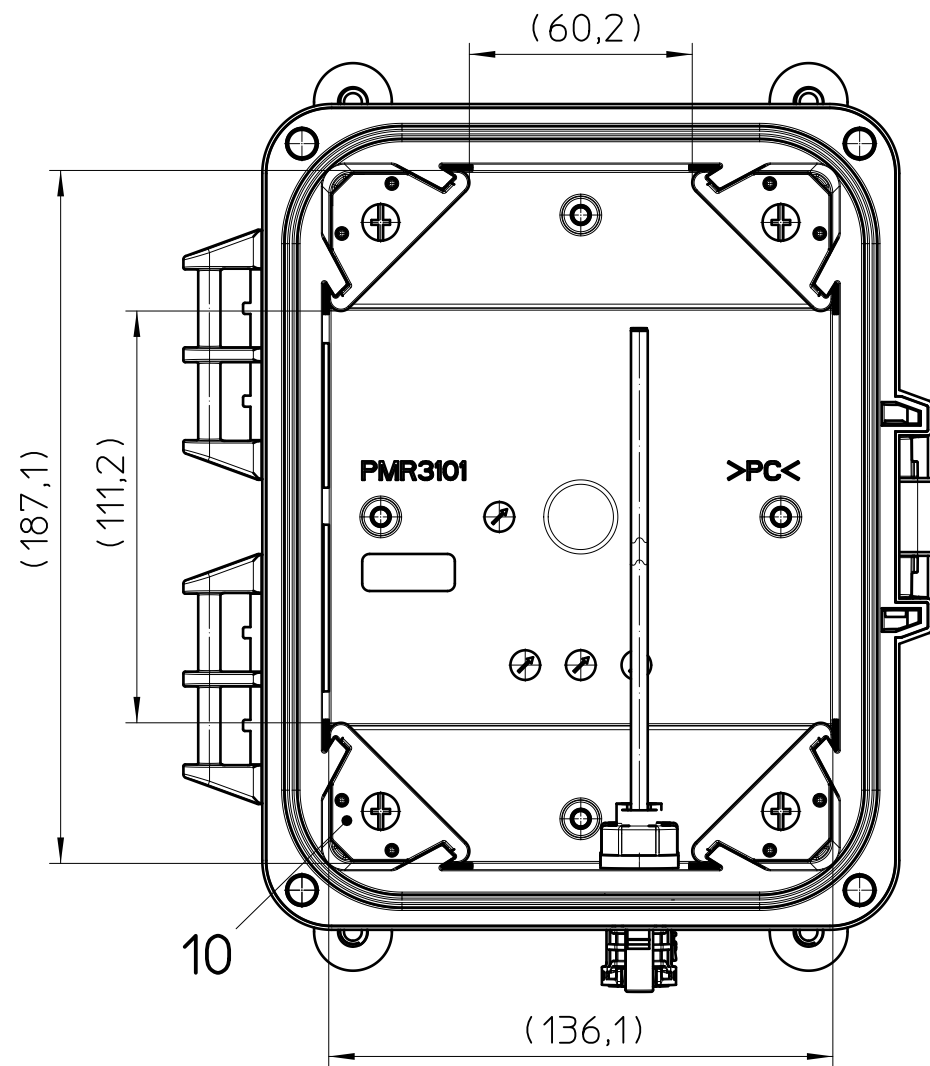
Front view without cover
