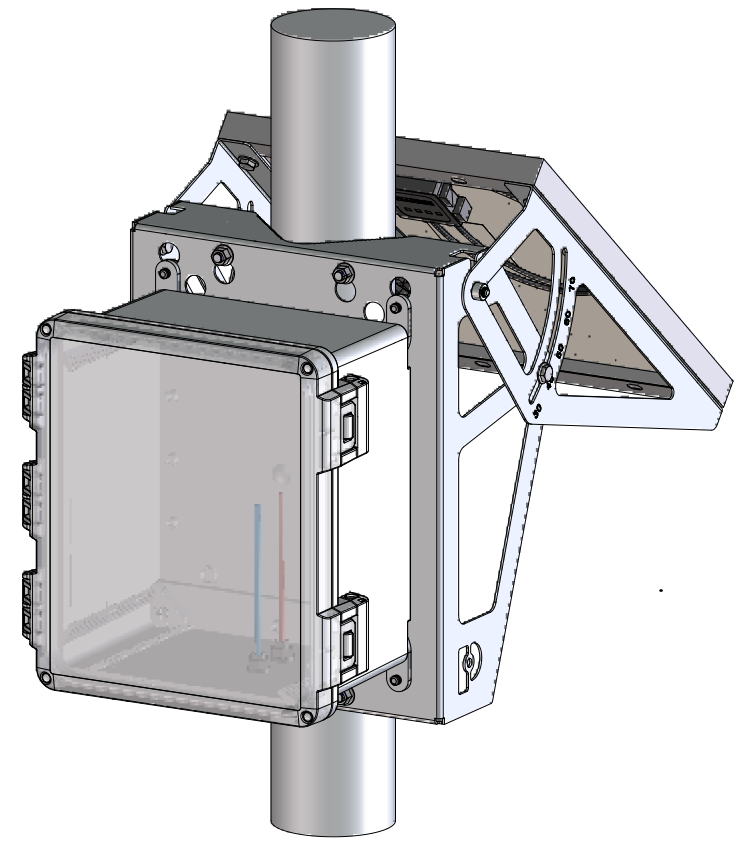
Assembly example
