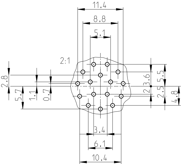
PCB-layout (advice)
