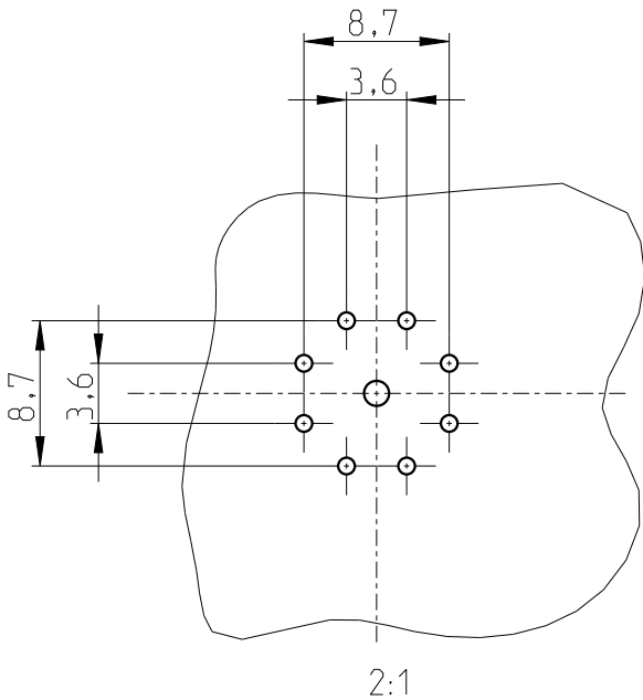
PCB-layout (advice)
