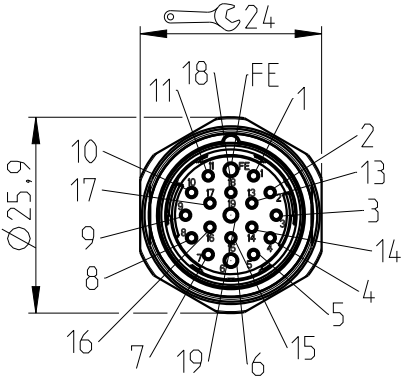
plug face male
