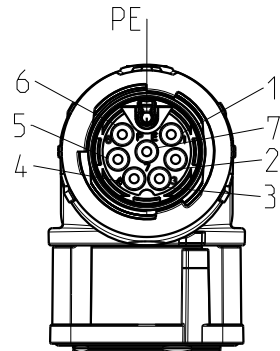
plug face male
