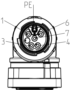
socket face female
