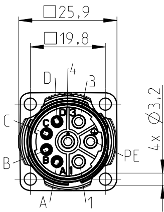
plug face male
