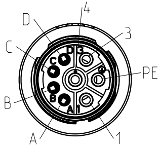
plug face male
