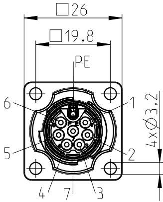
plug face male
