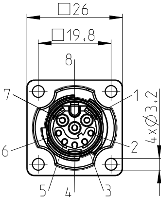
plug face male
