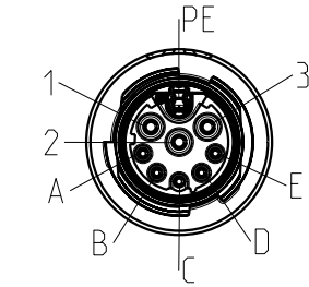
socket face female
