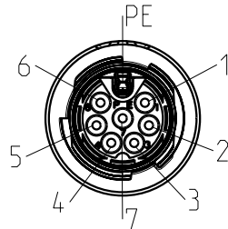
plug face male
