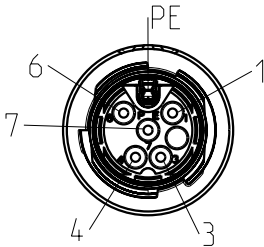
plug face male
