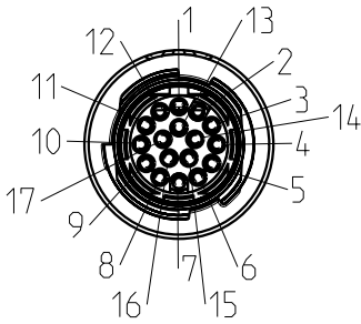
plug face male
