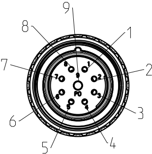
plug face male
