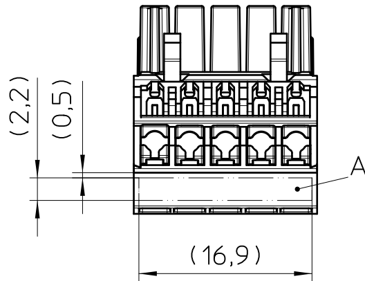
view X
