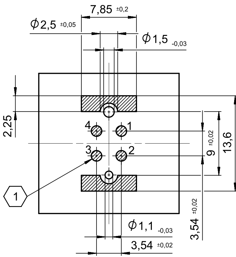
PCB-layout (advice)
