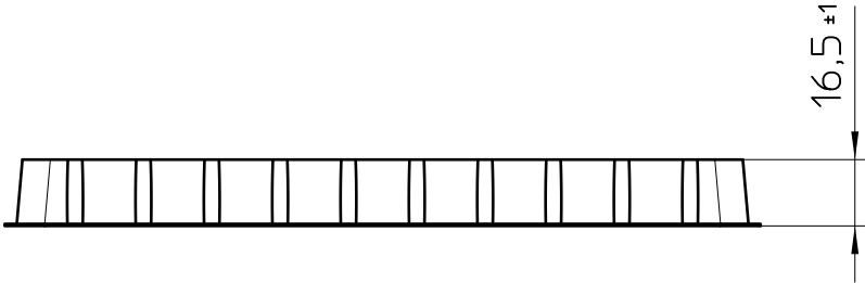
Packaging Tray
