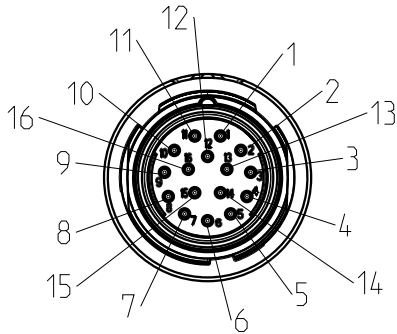
plug face male
