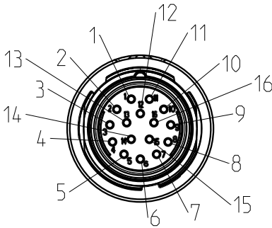
socket face female
