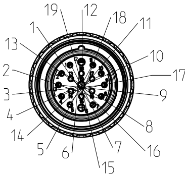
plug face female
