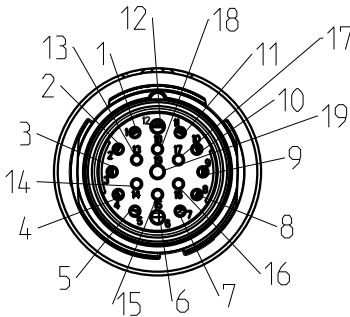
socket face female
