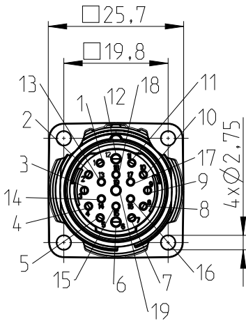
socket face female
