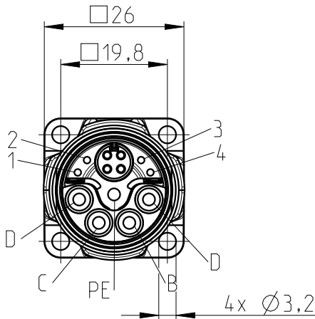
plug face male
