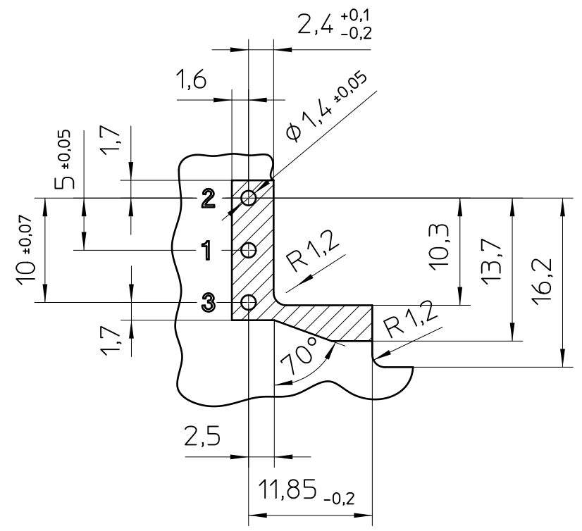
recommended PCB drilling plan view: component side
